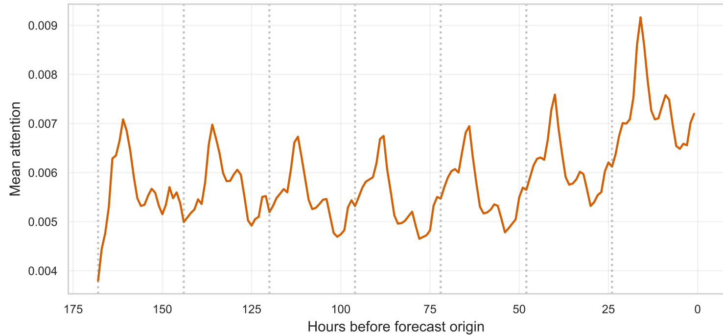
TFT temporal attention vs lag (test set, avg over horizon)
