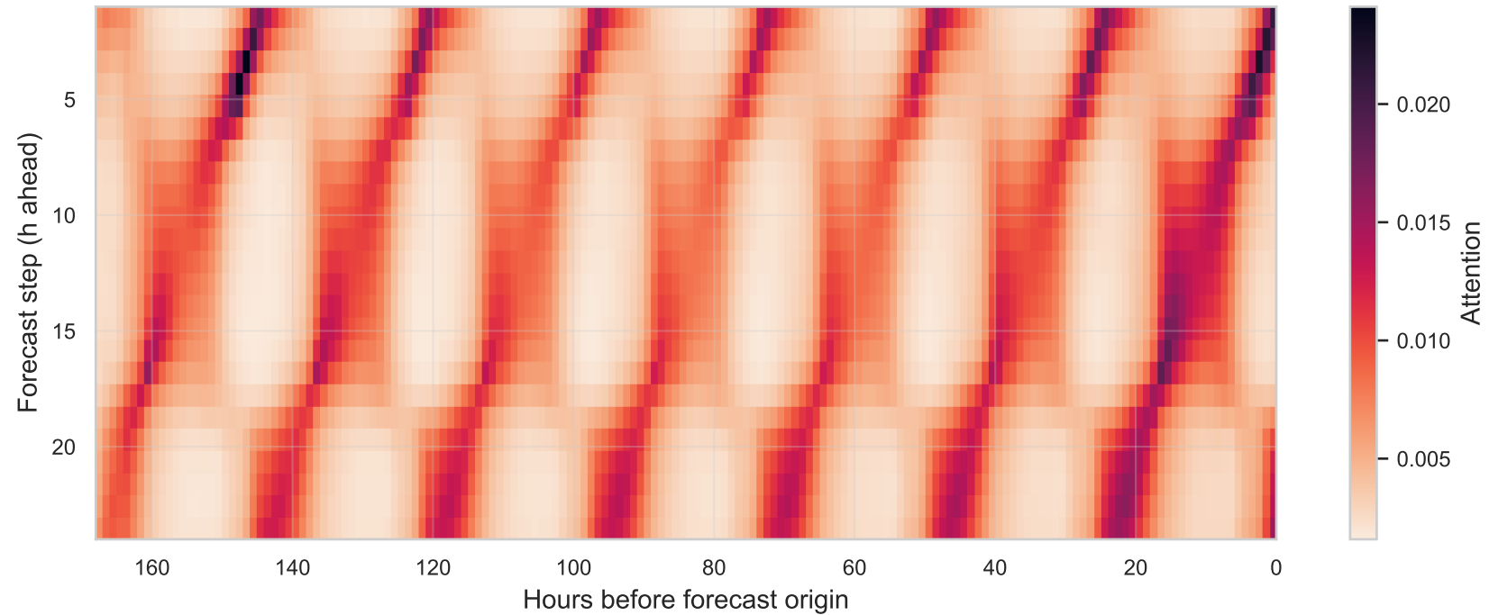
TFT attention heatmap (horizon step x hours before origin)
