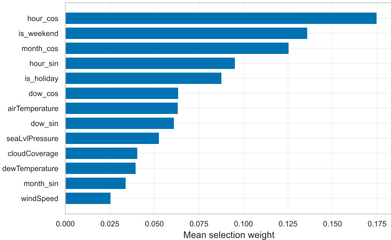
TFT variable selection - Decoder (future) inputs
