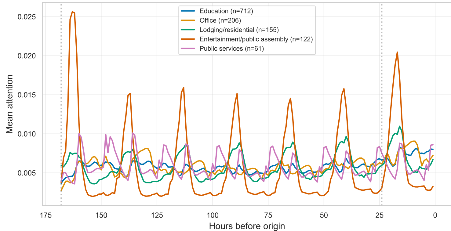
TFT attention vs lag by building type
