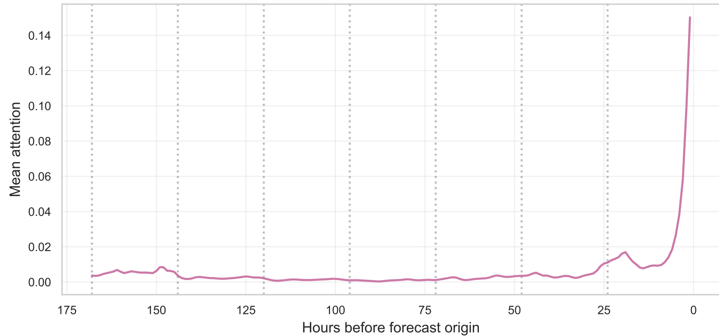
transformer attention vs lag (test set)
