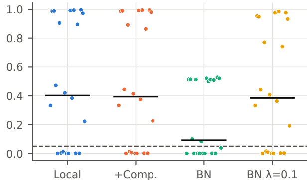
SO(3): ground-truth algebra distance (dashed: 'correct')
