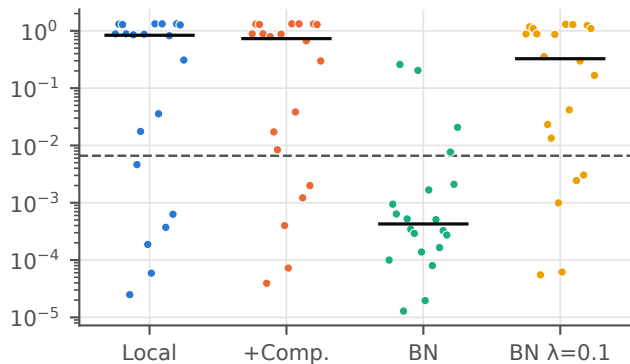
SO(3): ground-truth algebra distance (dashed: 'correct')
