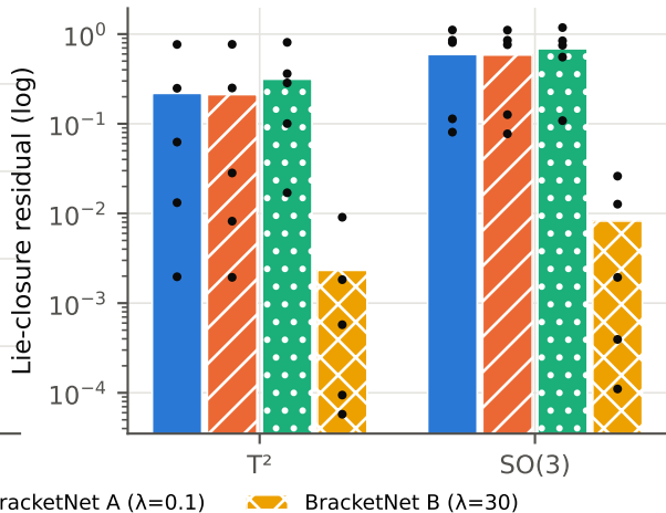
Algebraic fidelity (SO(2): identically 0)
