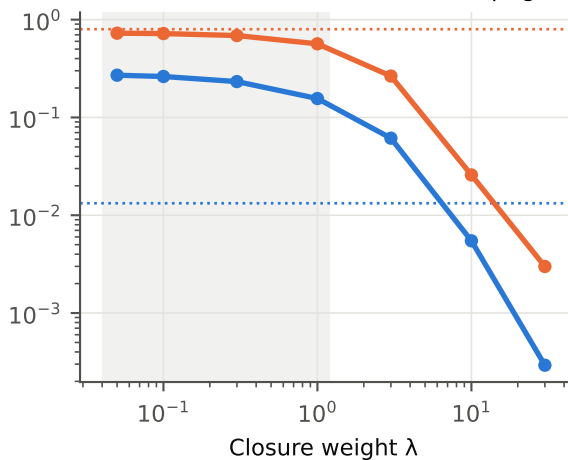
Validation closure (shaded: manuscript grid)
