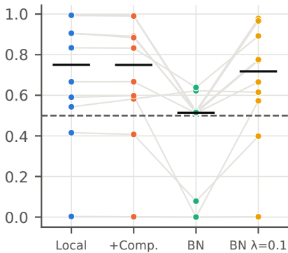
SO(3) : cross-seed algebra distance (10 disjoint pairs; dashed: random spans)
