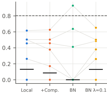
T^2 : cross-seed algebra distance (10 disjoint pairs; dashed: random spans)
