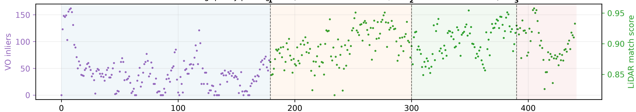
Front-end tracking quality per segment (visual = VO inlier count, LiDAR = scan-match score)
