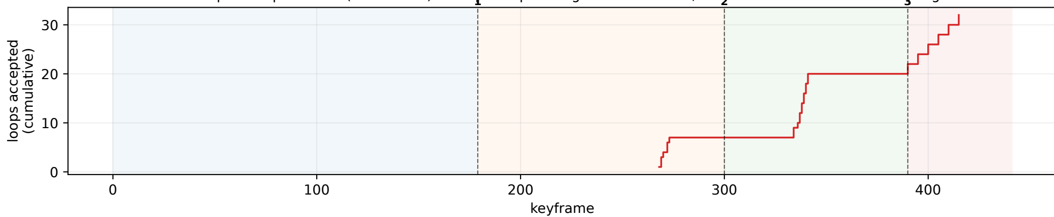
Accepted loop closures (cumulative) — loops keep closing across switches; flat stretches = route not revisiting
