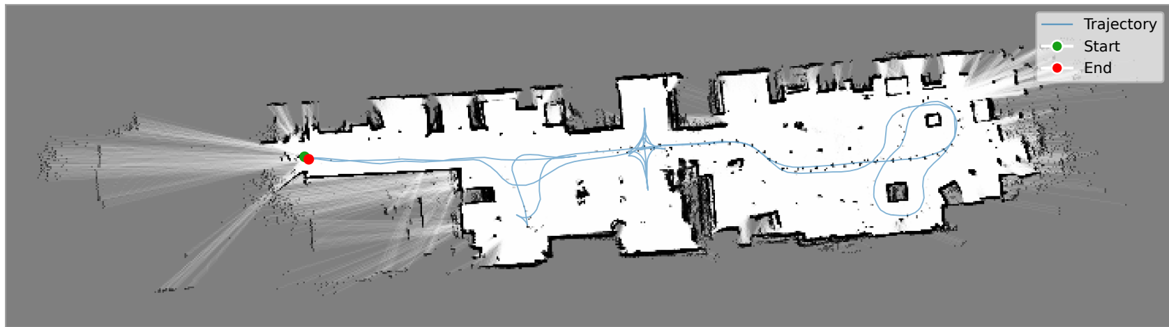
lab_2 (2 rooms) — LiDAR + visual-PnP · scan-to-map
