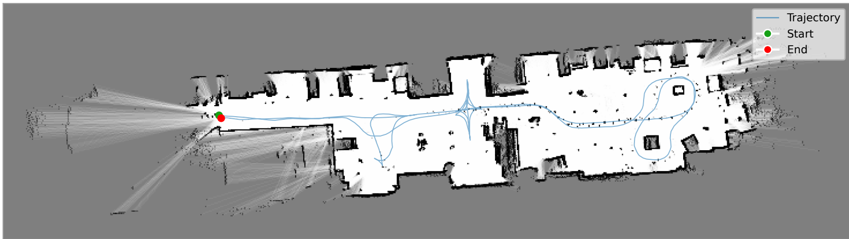
lab_2 (2 rooms) — LiDAR · scan-to-map · B&B
