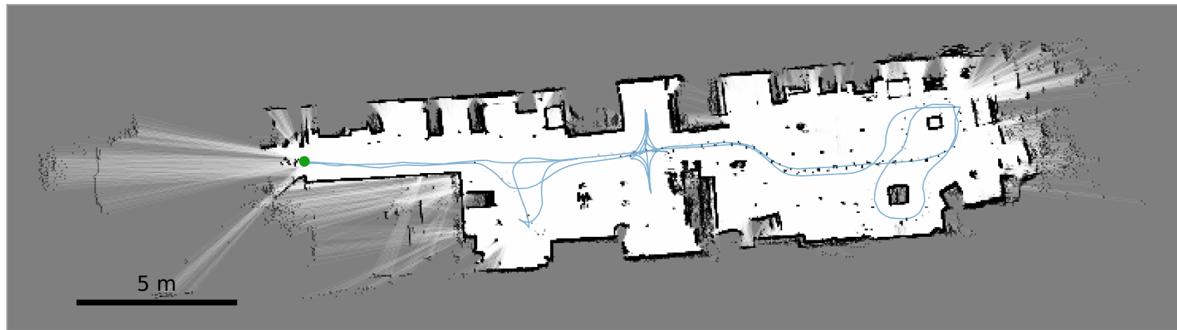
Two-room lab — LiDAR + visual-PnP · scan-to-map
