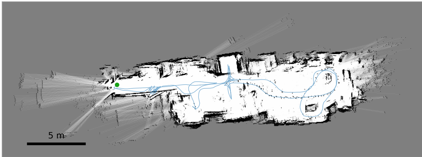
Two-room lab — LiDAR + visual-PnP · scan-to-submap
