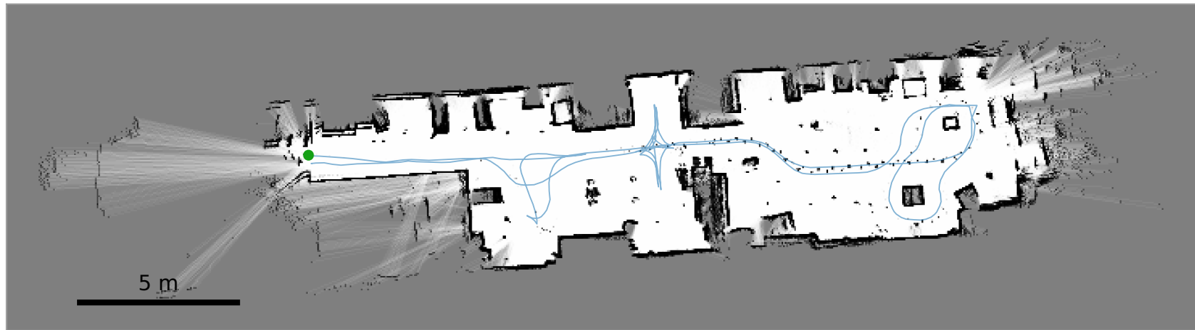
Two-room lab — LiDAR · scan-to-map · ICP
