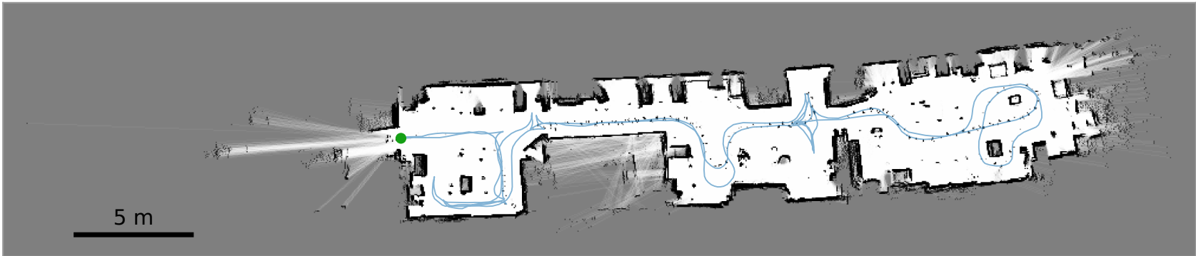
lab_hybrid_3 — LiDAR + visual-PnP · scan-to-map
