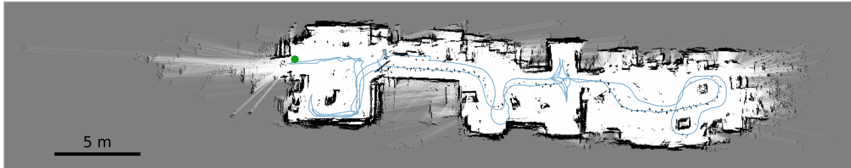
lab_hybrid_3 — LiDAR + visual-PnP · scan-to-submap
