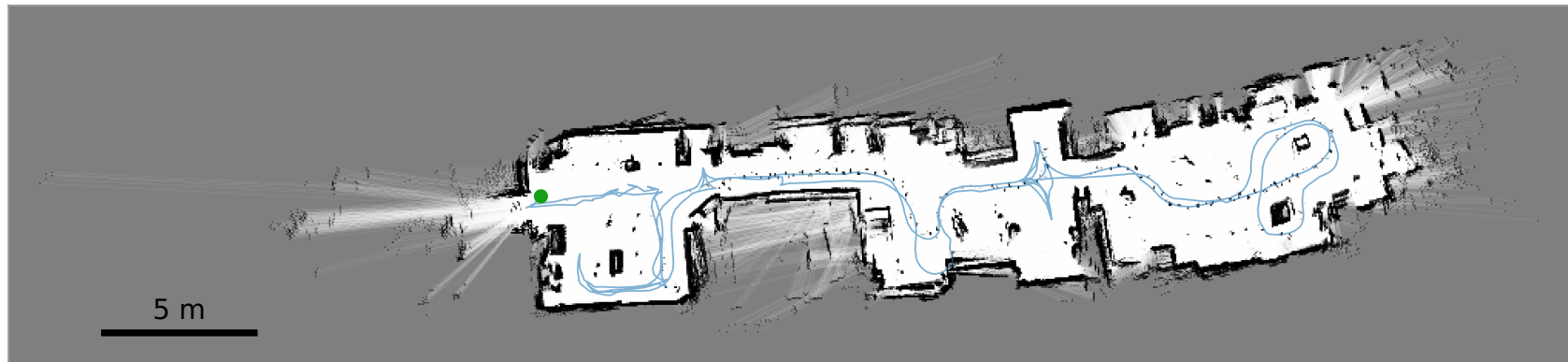
lab_hybrid_3 — LiDAR · scan-to-submap · B&B
