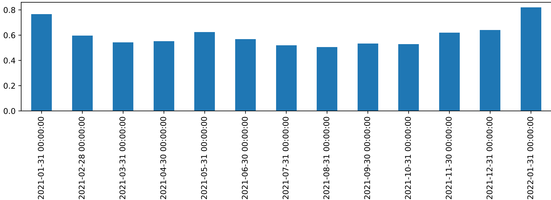
RMSE (monthly)
