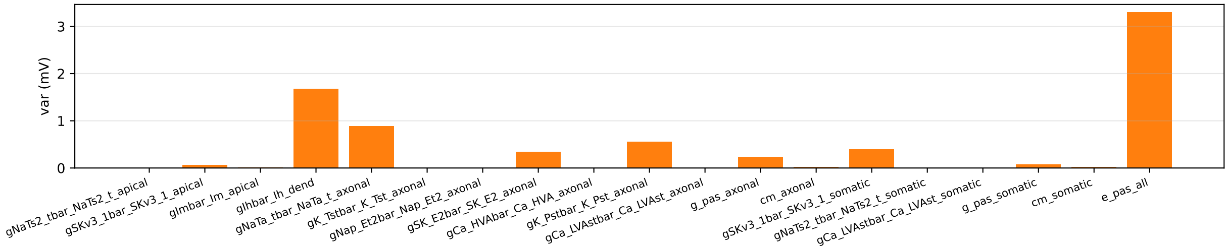
Roy1500_icaRec_5k @ x1 — per-channel voltage variation (sweep 1 channel over its box, hold rest at default)
