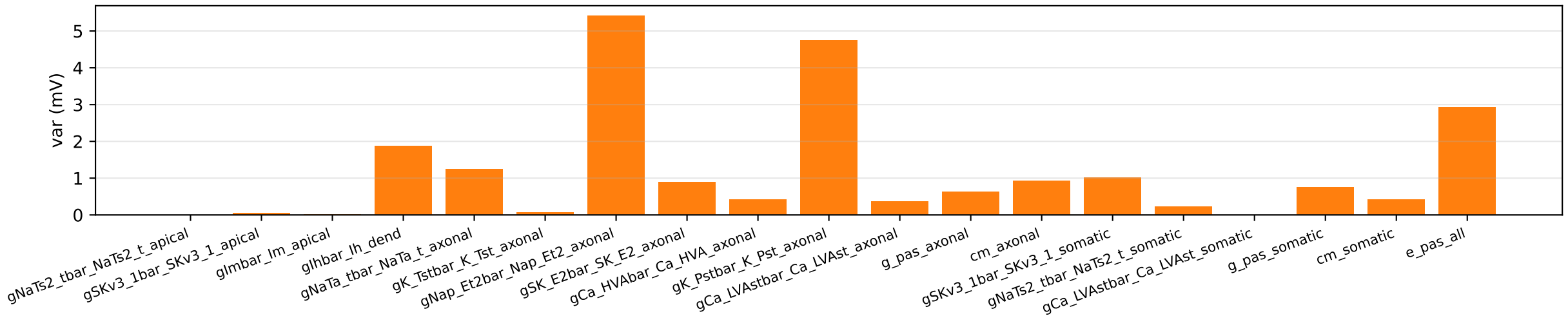
Roy2000_icaRec_5k @ x1 — per-channel voltage variation (sweep 1 channel over its box, hold rest at default)
