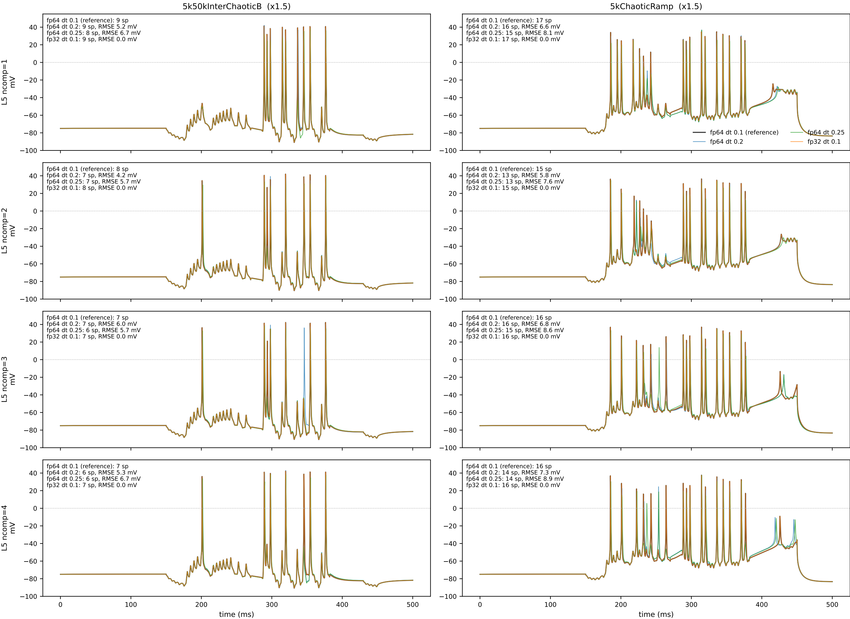
L5 default (BBP) parameters, soma voltage: solver precision / time-step variants overlaid, ncomp 1-4 per branch
