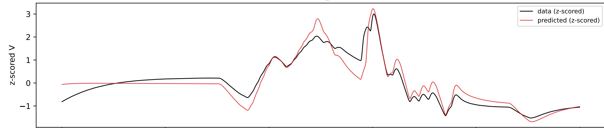
probe3 (5k50kInterChaoticB) rmse_z=0.394 spikes sim/data = 0/4
