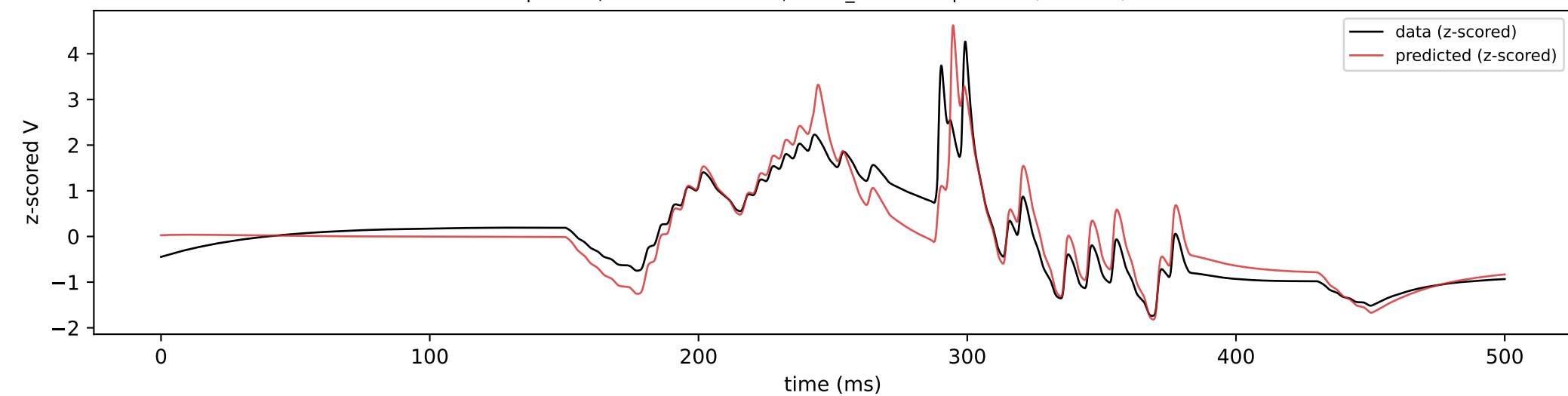
probe3 (5k50kInterChaoticB) rmse_z=0.394 spikes sim/data = 0/4
