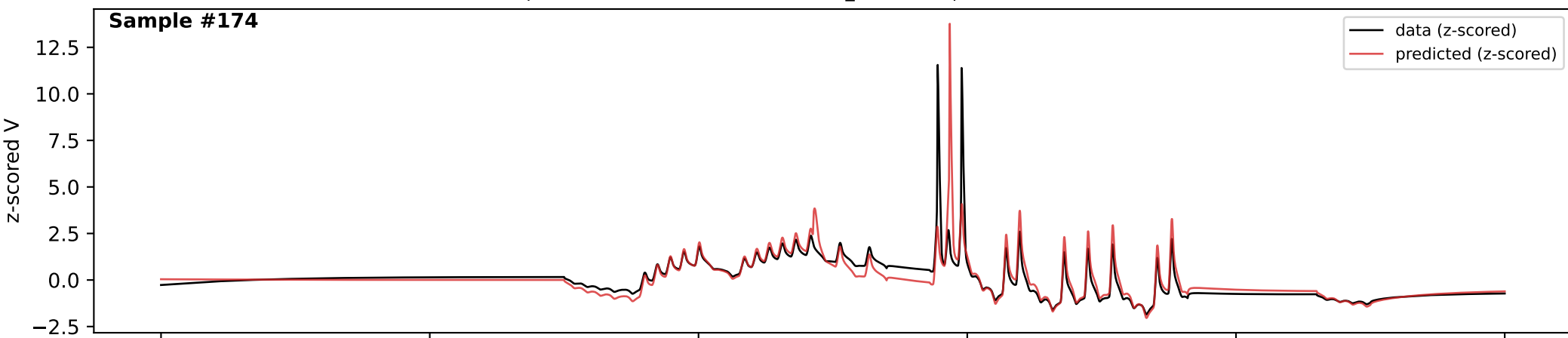
probe1 (5k50kInterChaoticB) rmse_z=0.956 spikes sim/data = 2/6
