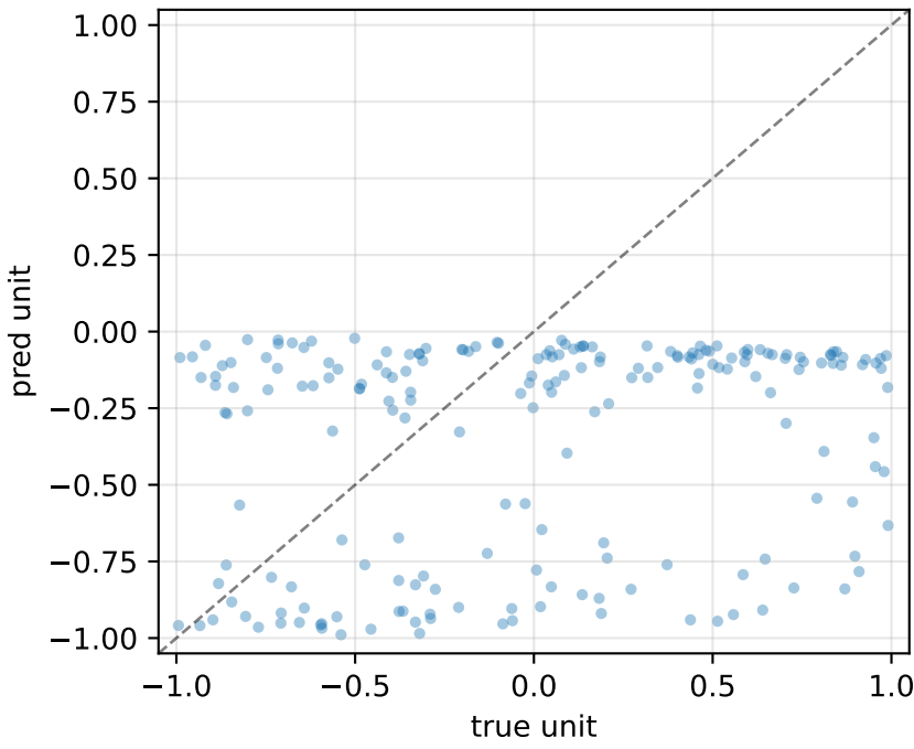
g_pas_somatic R^2=-0.64 MSE=0.564
