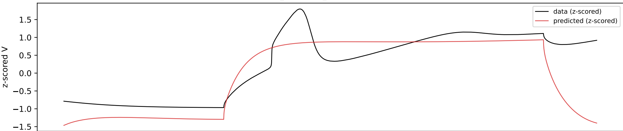
probe1 (5k0step_500) rmse_z=0.652 spikes sim/data = 0/0
