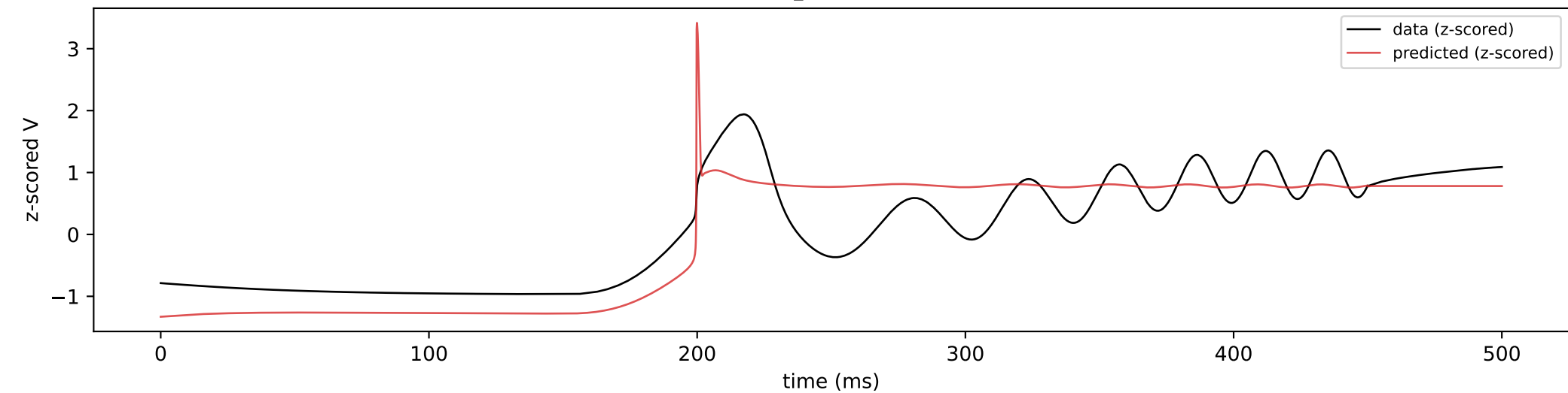
probe2 (5k0chirp) rmse_z=0.470 spikes sim/data = 1/0
