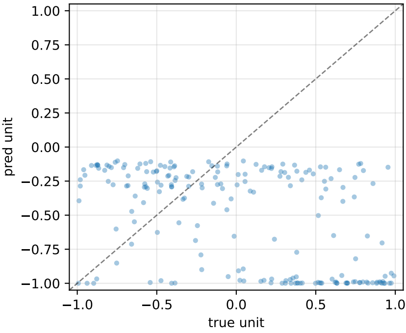
gK_Pstbar_K_Pst_axonal R^2=-1.79 MSE=0.998
