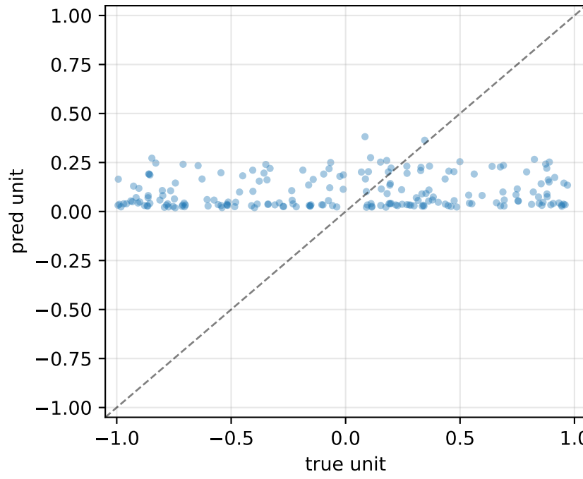
g_pas_axonal R^2=-0.38 MSE=0.496
