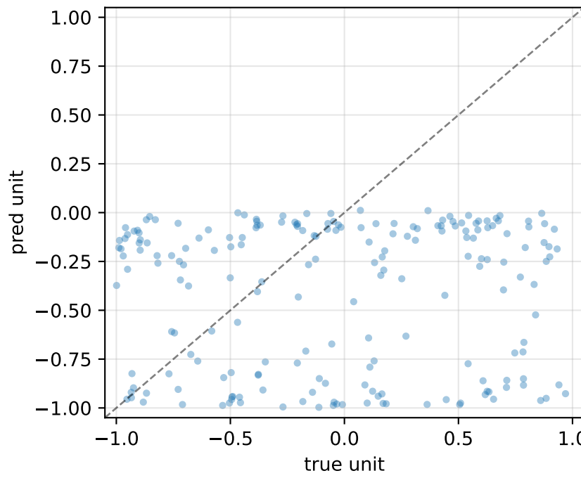
cm_somatic R^2=-0.77 MSE=0.618
