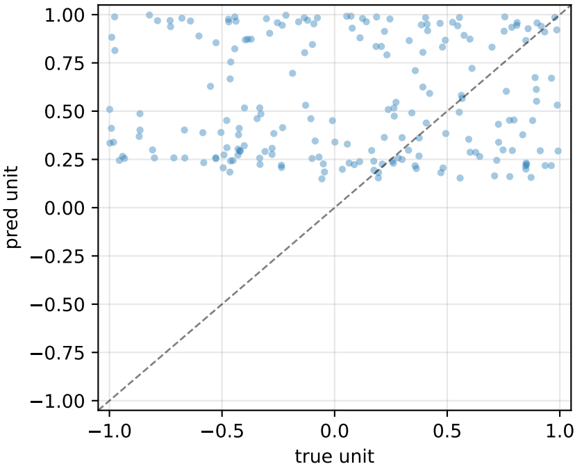
gNap_Et2bar_Nap_Et2_axonal R^2=-1.78 MSE=0.954
