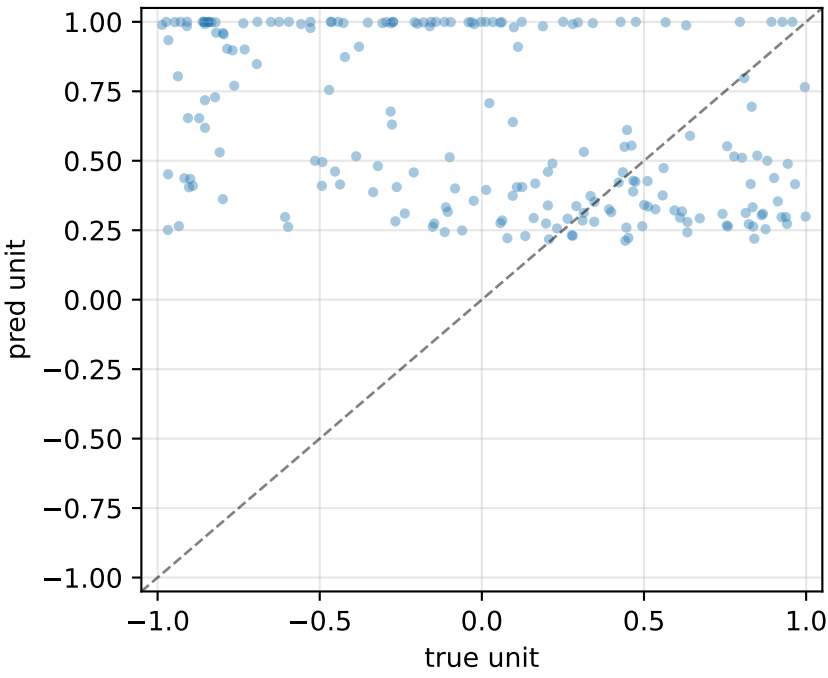
cm_axonal R^2=-1.32 MSE=0.780
