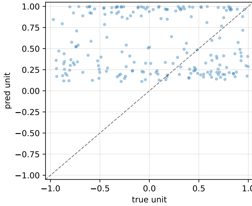
gCa_HVAbar_Ca_HVA_axonal R^2=-0.02 MSE=0.359
