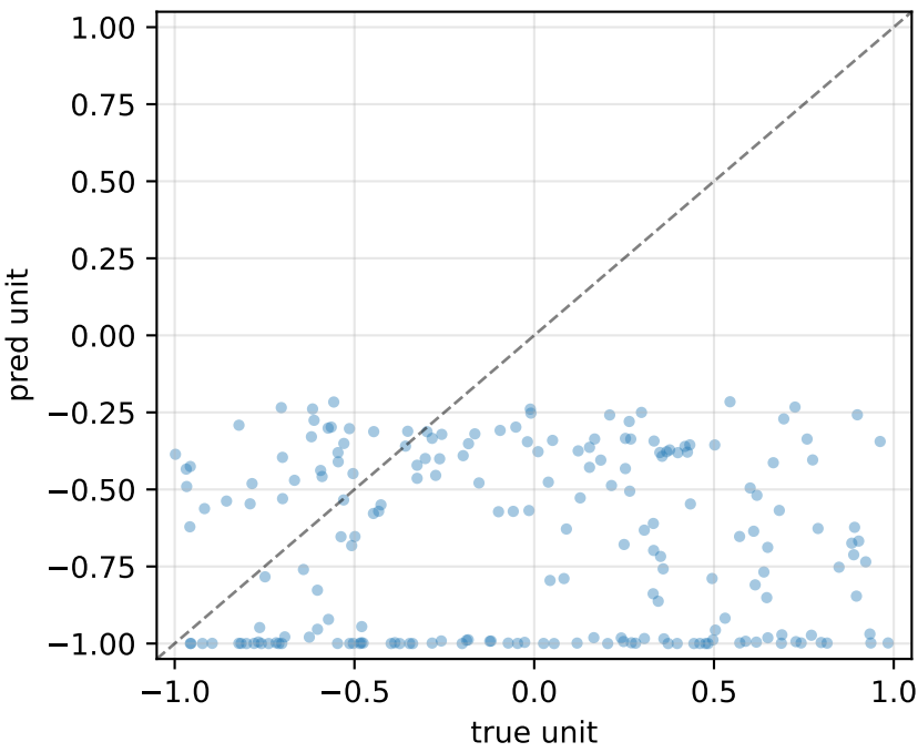
e_pas_all R^2=-1.67 MSE=0.818
