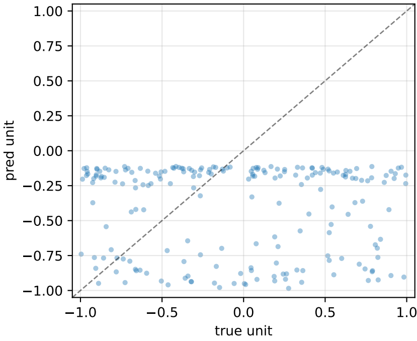
gSKv3_1bar_SKv3_1_somatic R^2=-0.49 MSE=0.500
