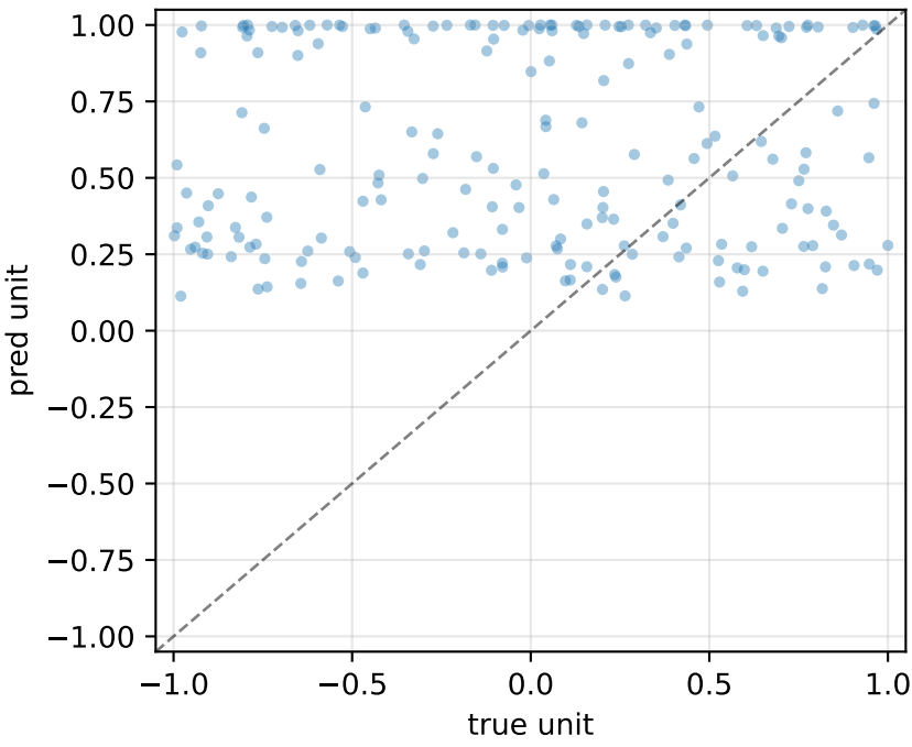
gCa_LVAstbar_Ca_LVAst_somatic R^2=-0.01 MSE=0.307
