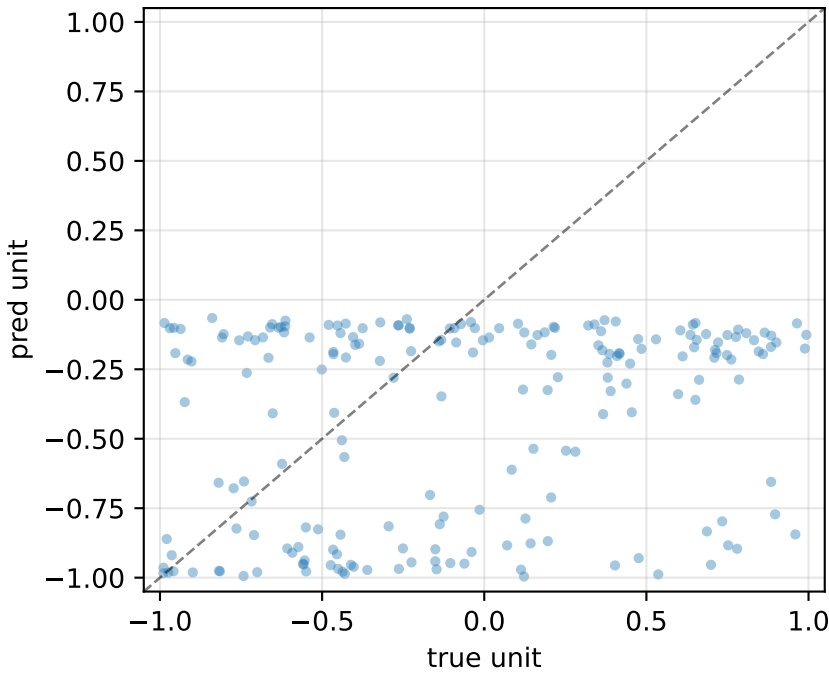
gCa_LVAstbar_Ca_LVAst_axonal R^2=-0.73 MSE=0.607
