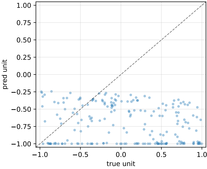
gSK_E2bar_SK_E2_axonal R^2=-0.49 MSE=0.489
