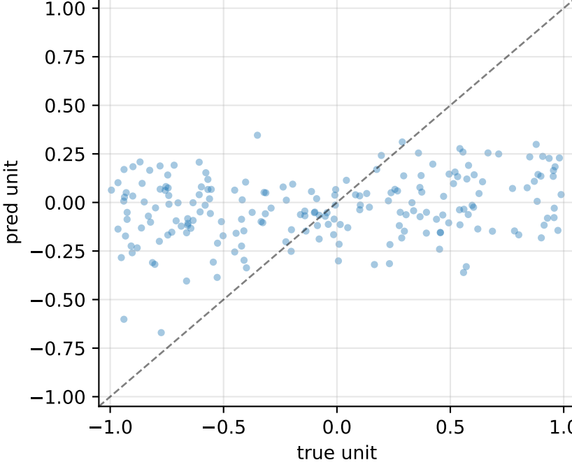
gCa_LVAstbar_Ca_LVAst_somatic R^2=+0.00 MSE=0.276
