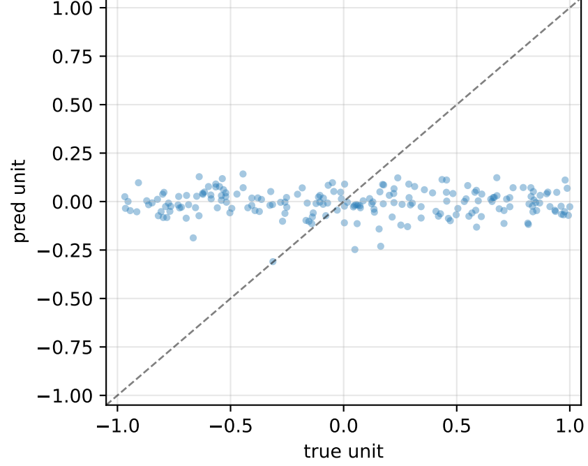
gCa_HVAbar_Ca_HVA_axonal R^2=+0.11 MSE=0.309
