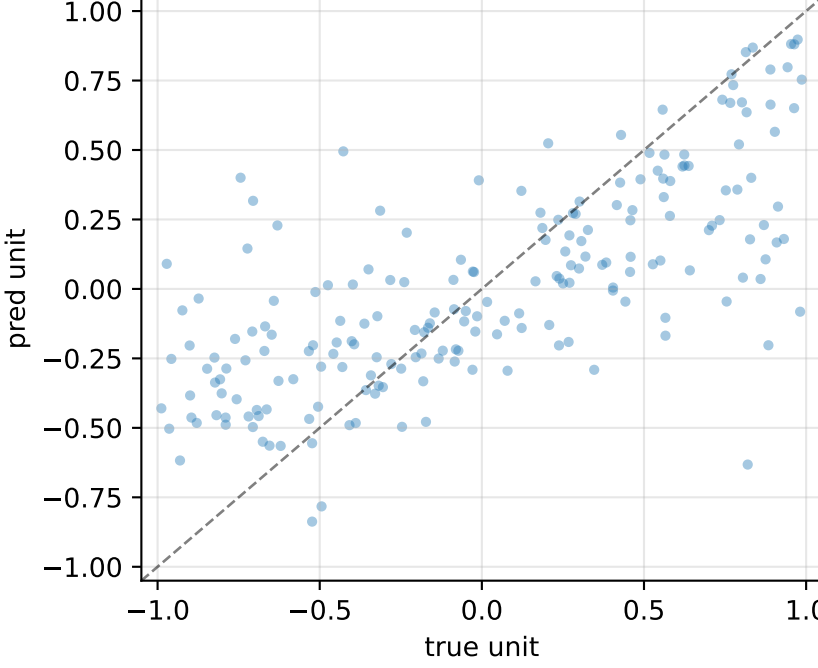
gNap_Et2bar_Nap_Et2_axonal R^2=+0.22 MSE=0.228
