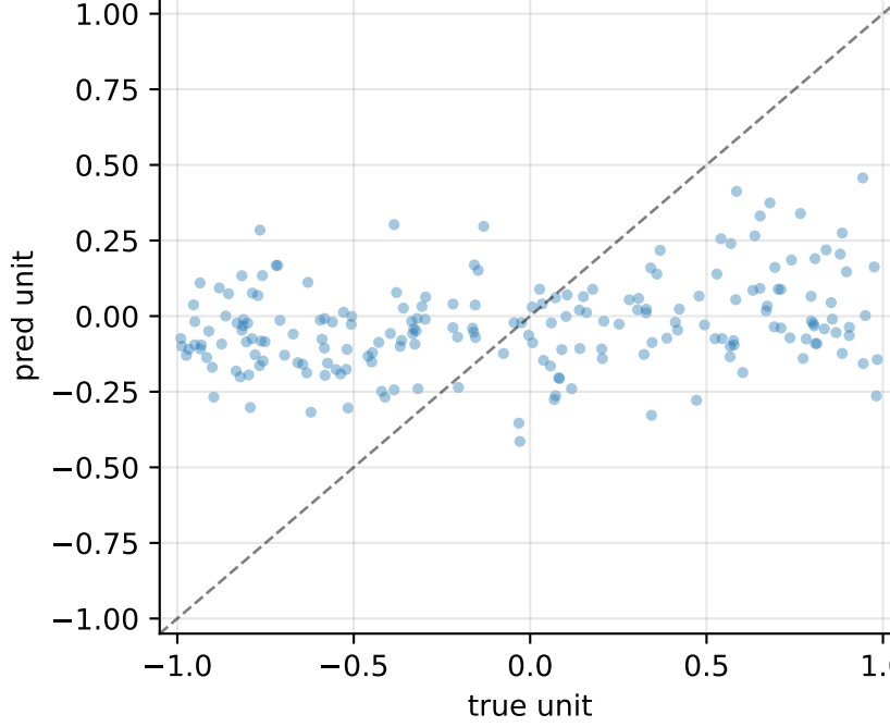
g_pas_somatic R^2=+0.08 MSE=0.343
