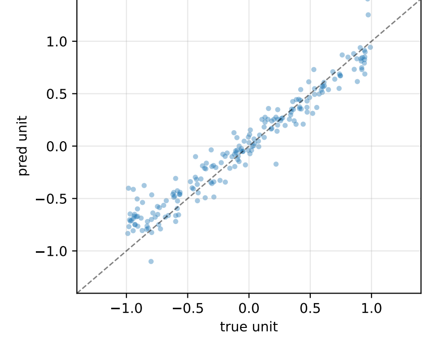
cm_somatic R^2=+0.53 MSE=0.165
