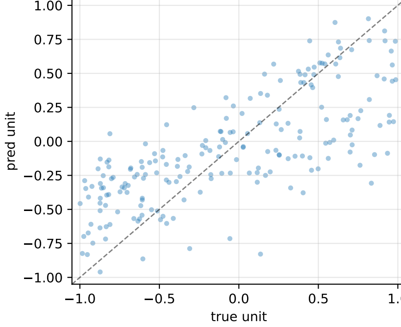
gCa_LVAstbar_Ca_LVAst_axonal R^2=+0.14 MSE=0.280
