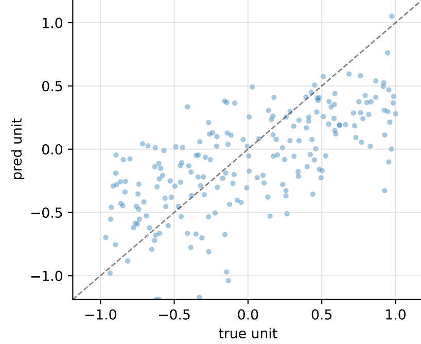
cm_axonal R^2=+0.06 MSE=0.340
