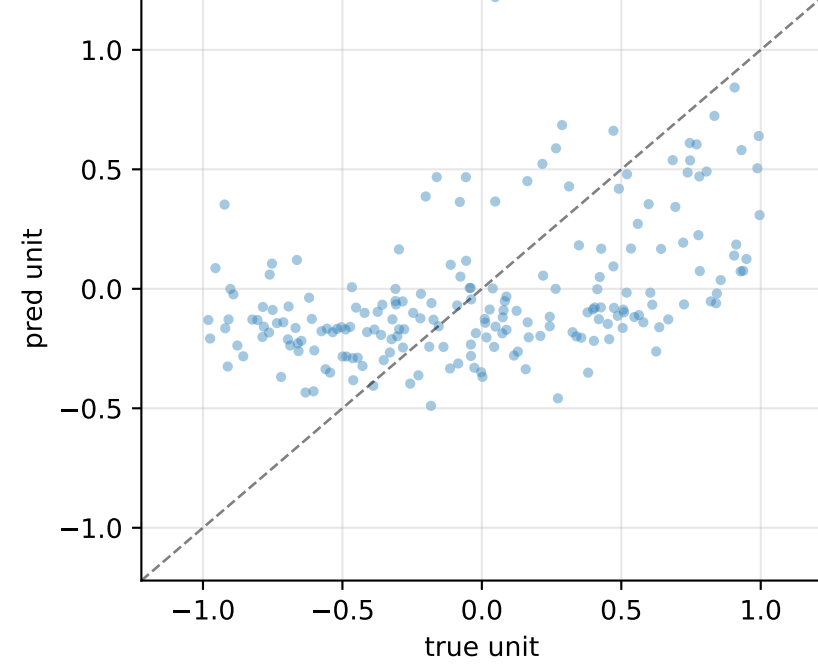
gK_Pstbar_K_Pst_axonal R^2=+0.43 MSE=0.187
