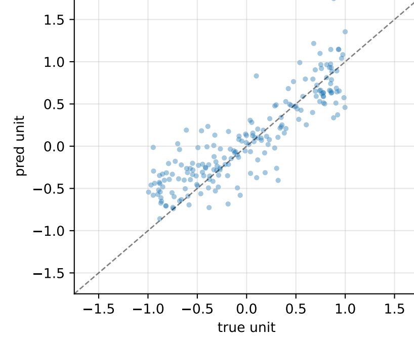
gSK_E2bar_SK_E2_axonal R^2=+0.54 MSE=0.168
