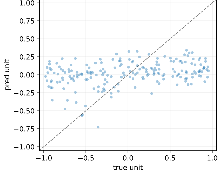
g_pas_axonal R^2=+0.05 MSE=0.341
