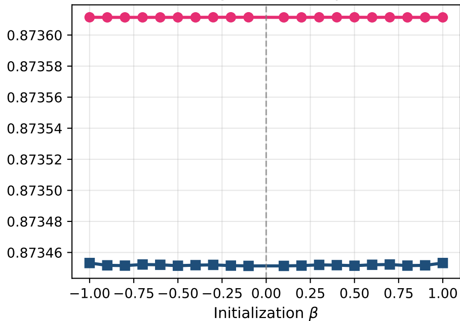
Weighted Accuracy
