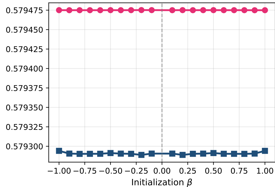
Kendall's Tau
