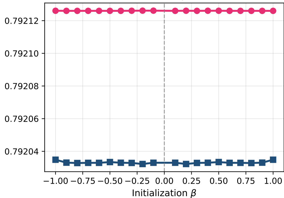
Accuracy
