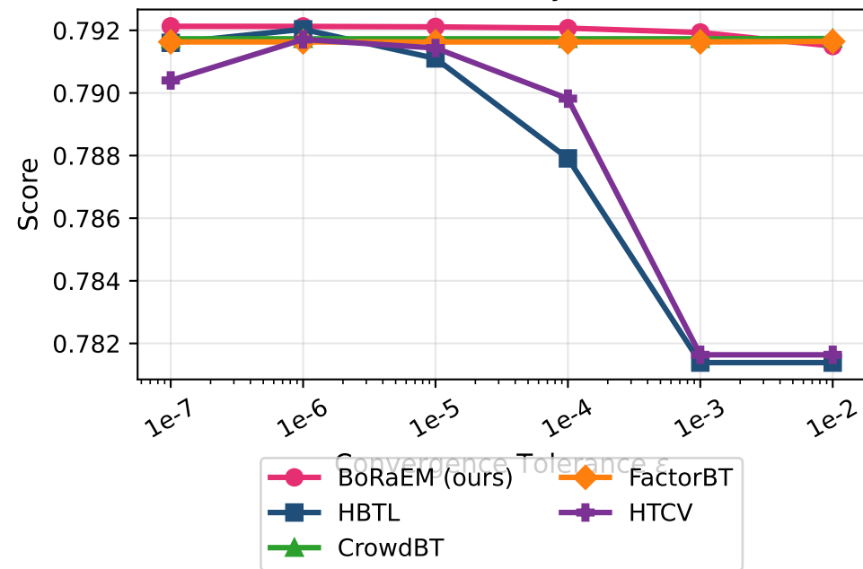
Accuracy
