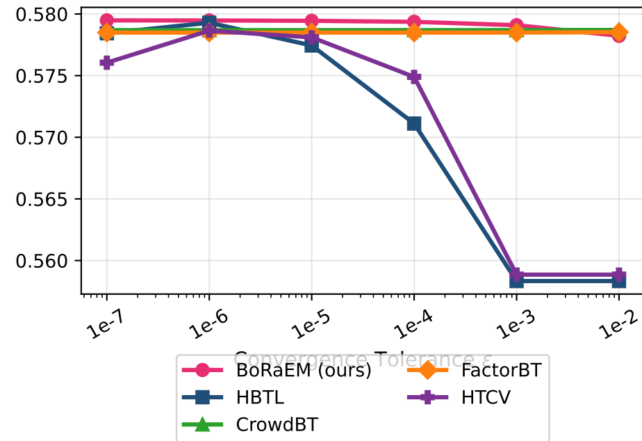
Kendall's Tau
