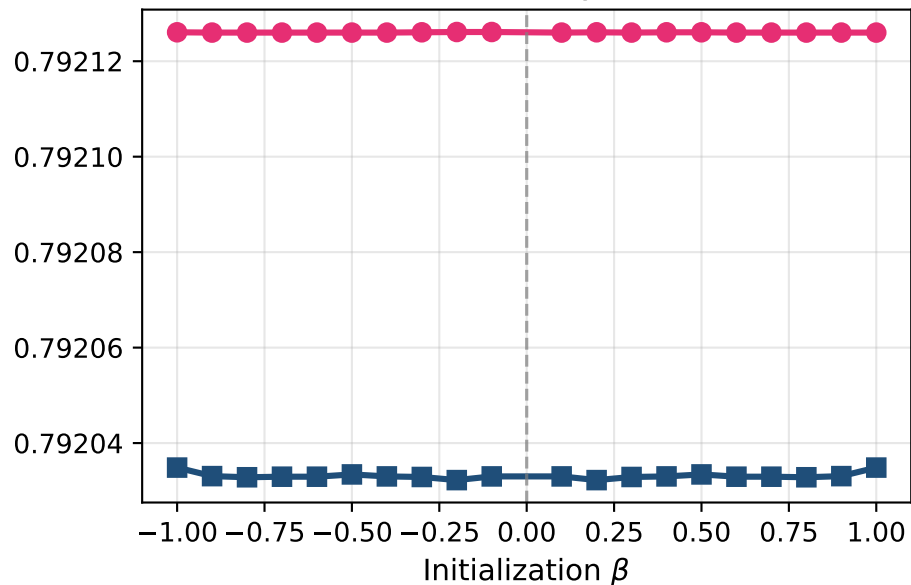
Accuracy
