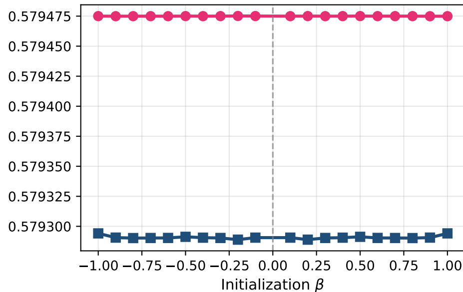
Kendall's Tau
