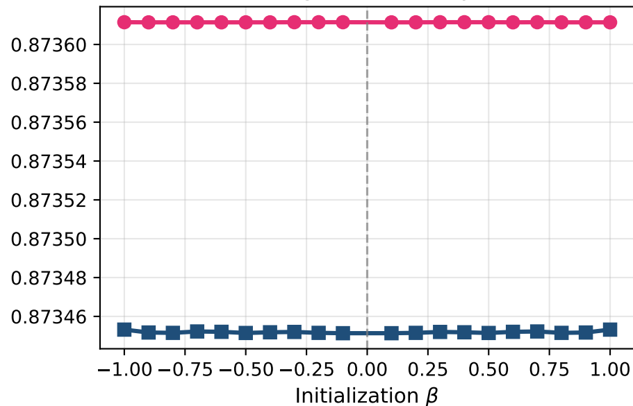
Weighted Accuracy
