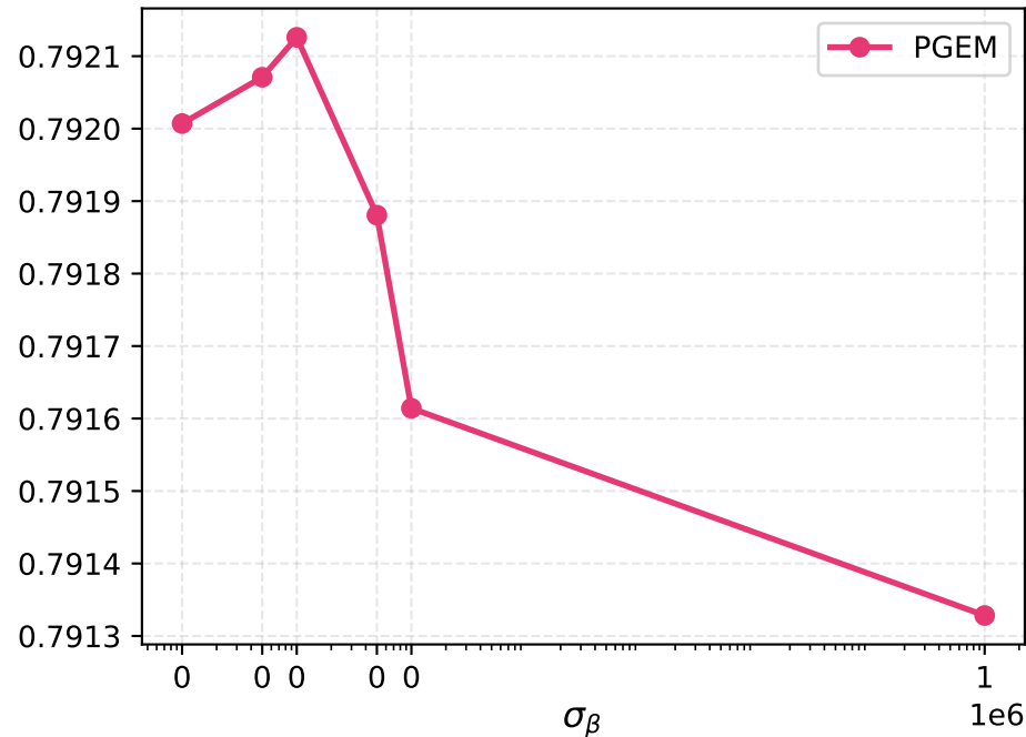
Accuracy
