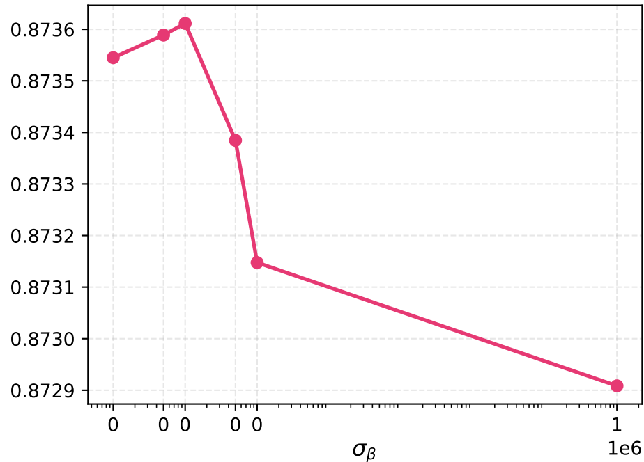
Weighted Accuracy
