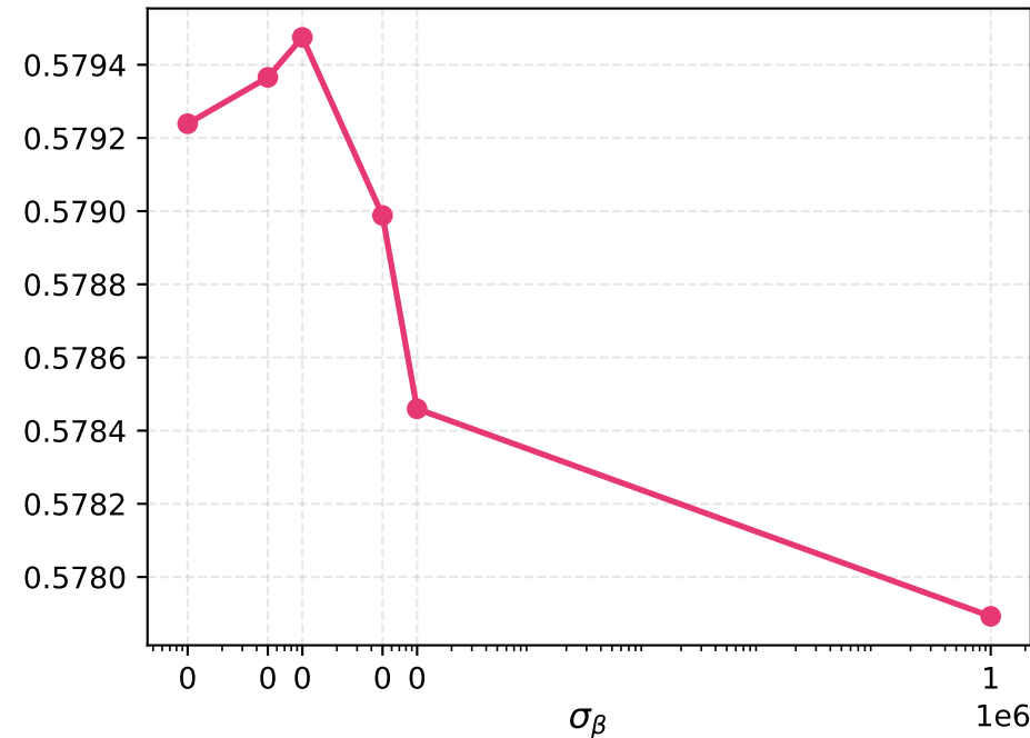
Kendall's Tau
