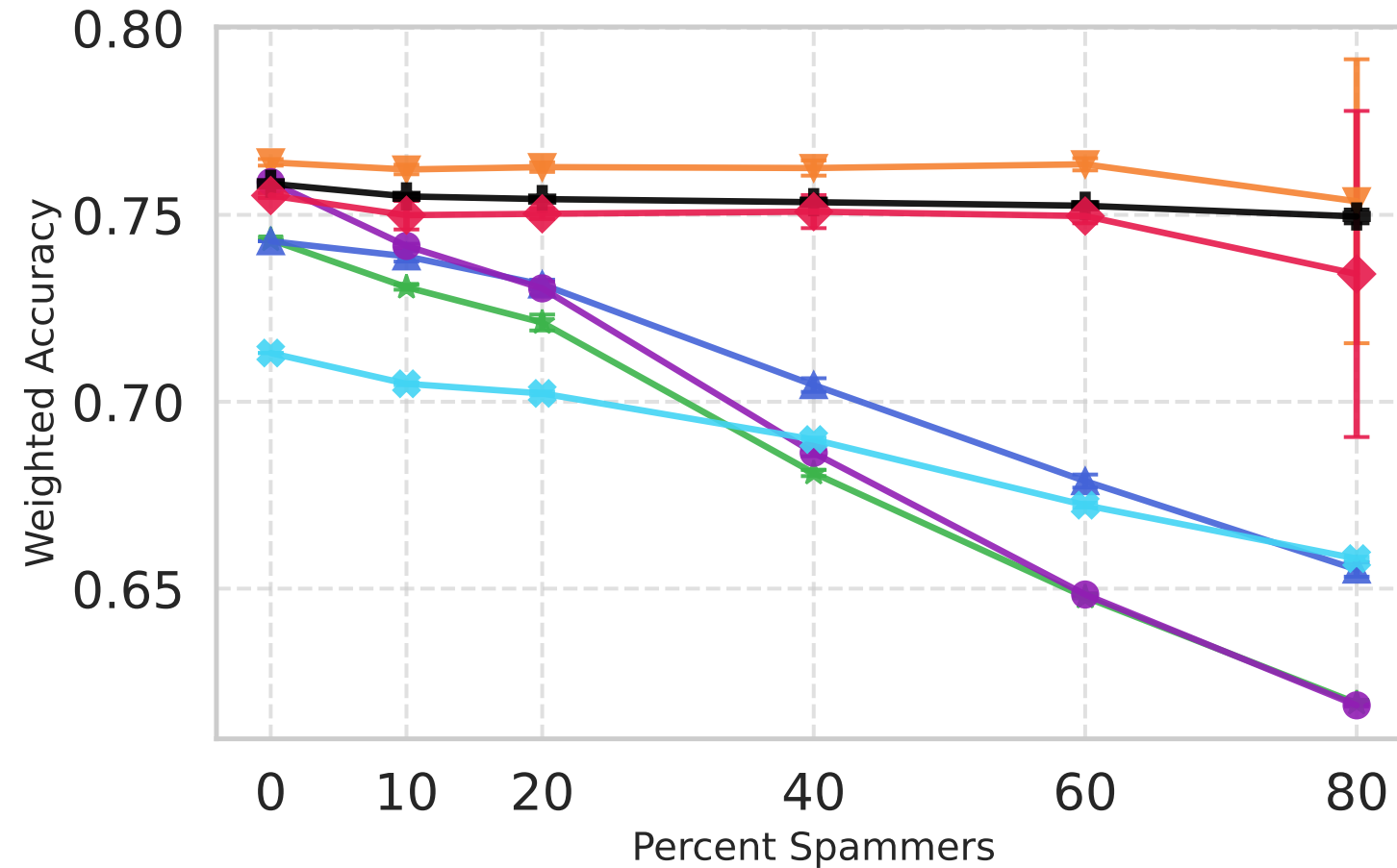
Adding left-position biased spammers
