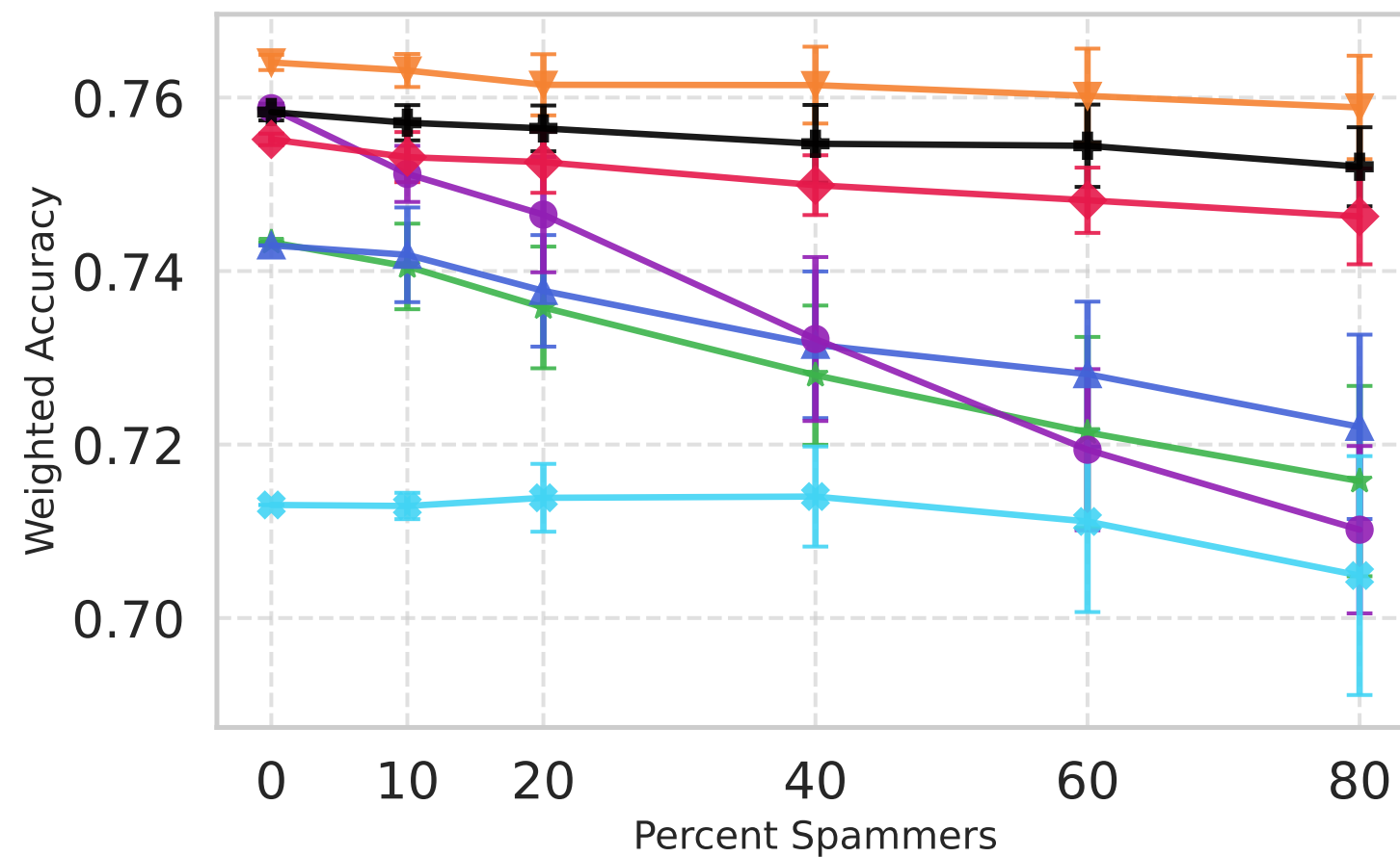
Adding all four types of spammers uniformly
