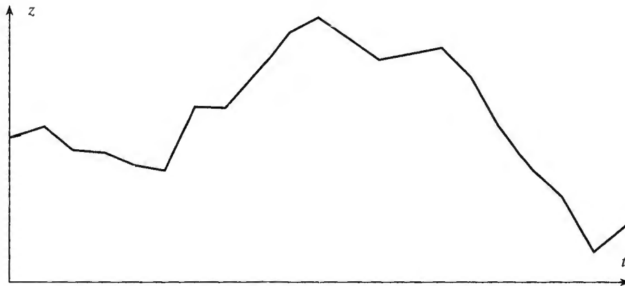
Figure 13.1 How a Wiener process is obtained when \Delta t \rightarrow 0 in equation (12.1).
