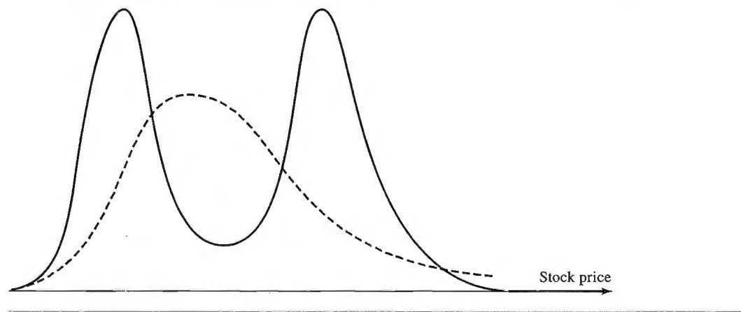
Figure 19.5 Effect of a single large jump. The solid line is the true distribution; the dashed line is the lognormal distribution.
