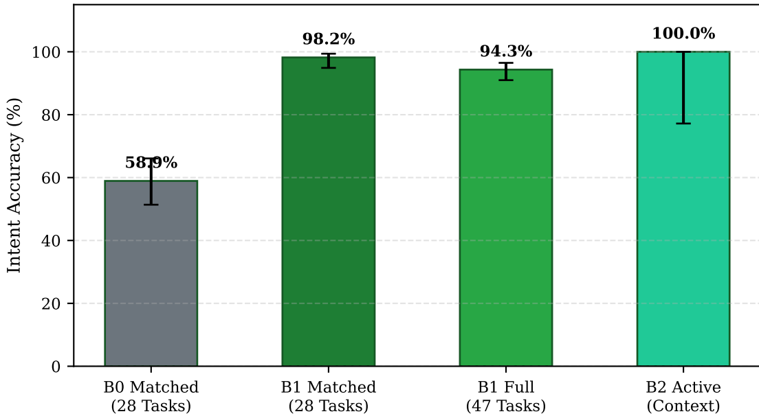
Intent Classification Accuracy (Wilson 95% CI)
