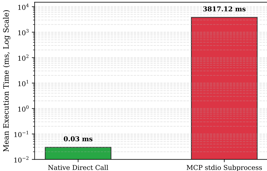
Current MCP Subprocess Launch Overhead Profile
