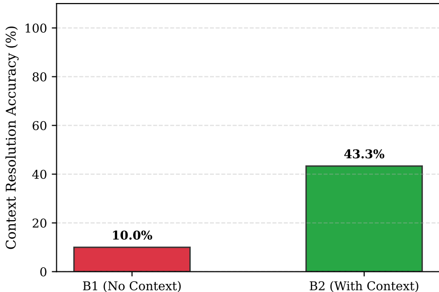
RQ2: Context Resolution Accuracy (B1 vs B2)
