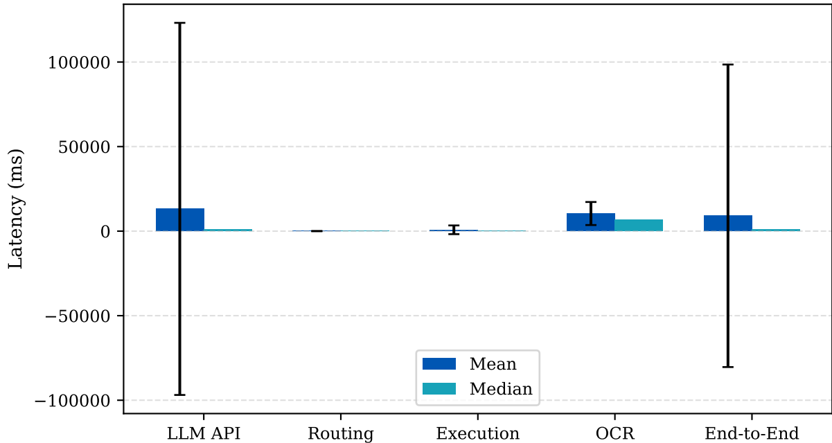
Latency Breakdown by Processing Stage
