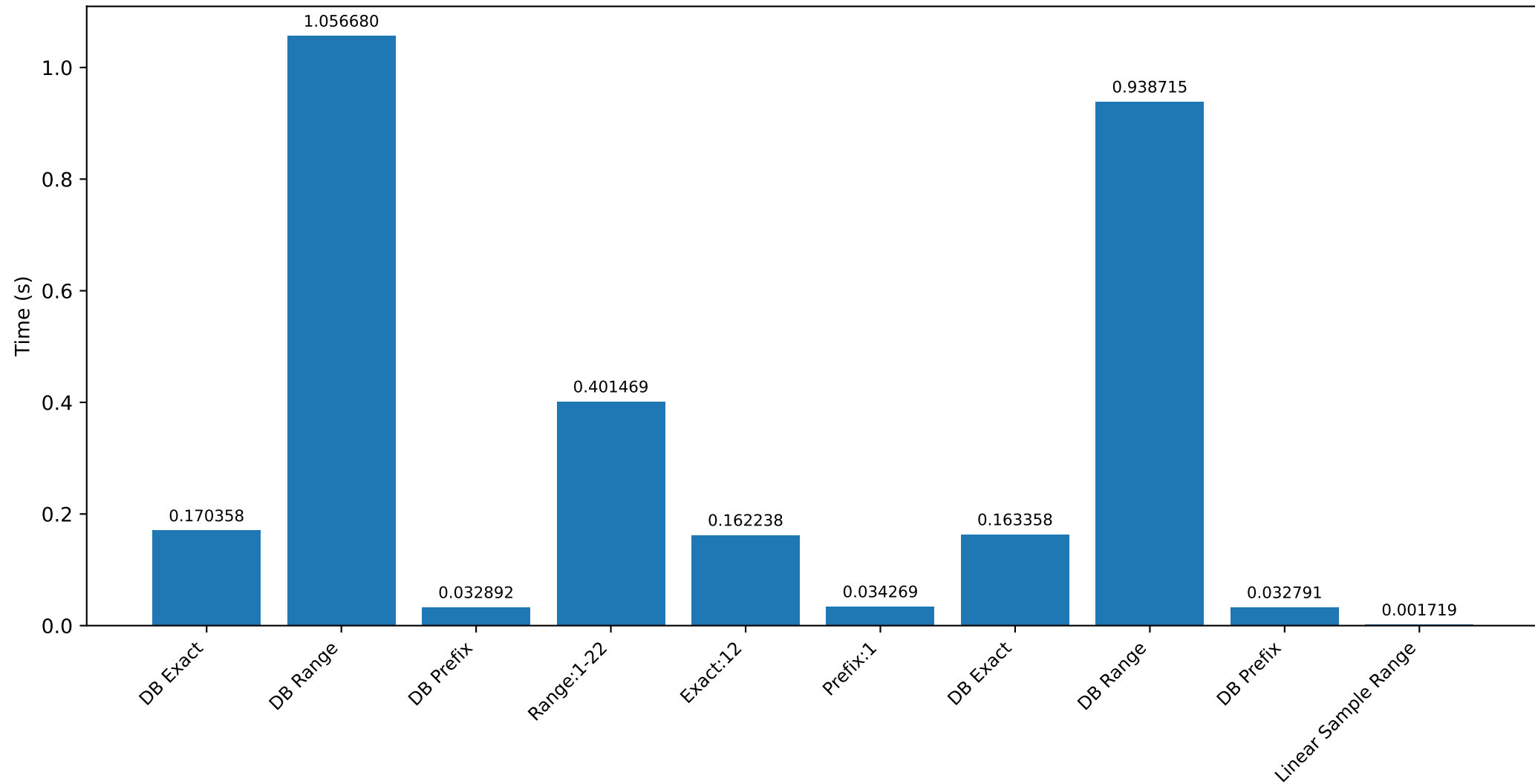
Method timings
