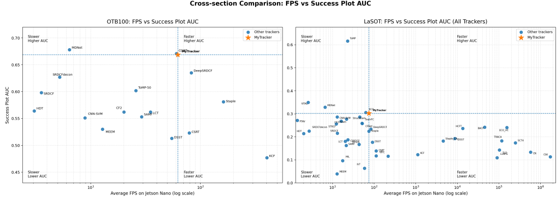
Figure 3: Cross-dataset FPS–AUC comparison on OTB100 and the evaluated LaSOT subset. The figure is used to analyze the accuracy-speed trade-off rather than to claim absolute superiority in a single metric.
