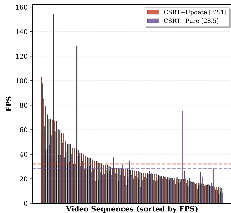
Speed Comparison (Frames Per Second)
