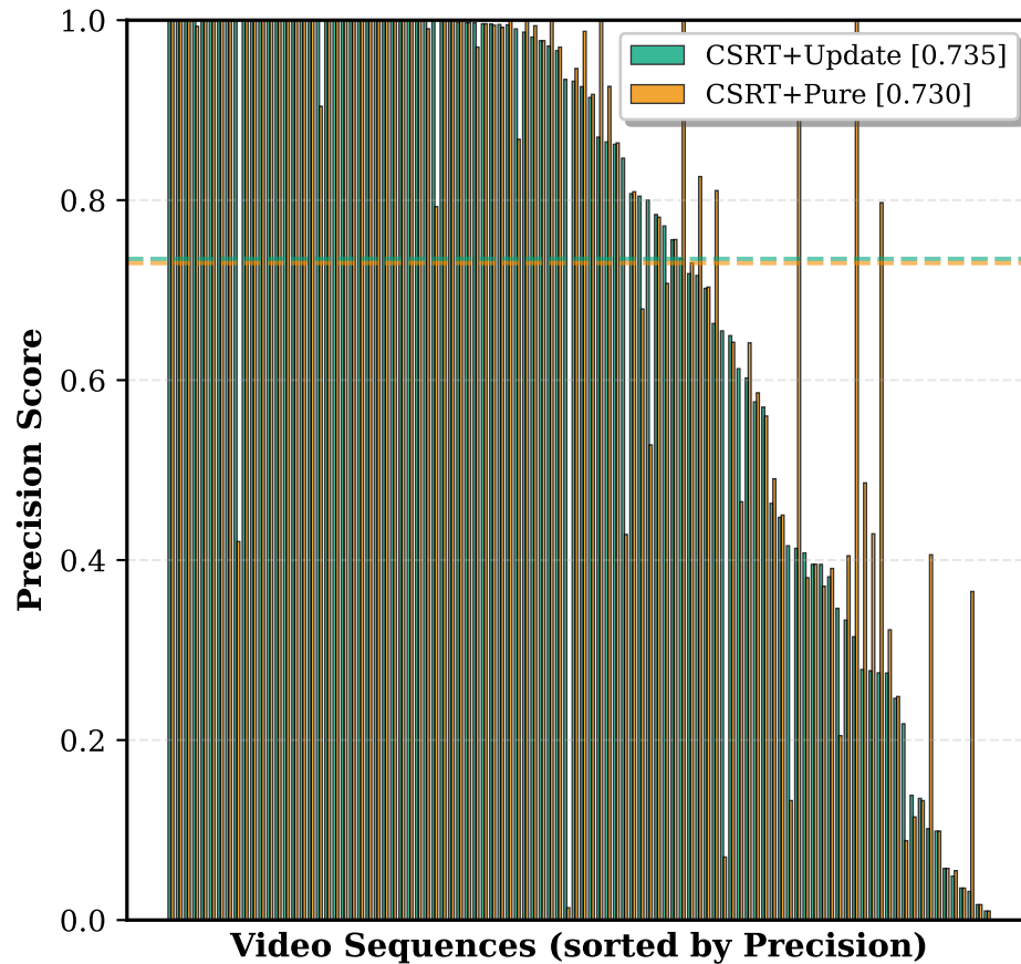
Precision Plot @ 20 pixels
