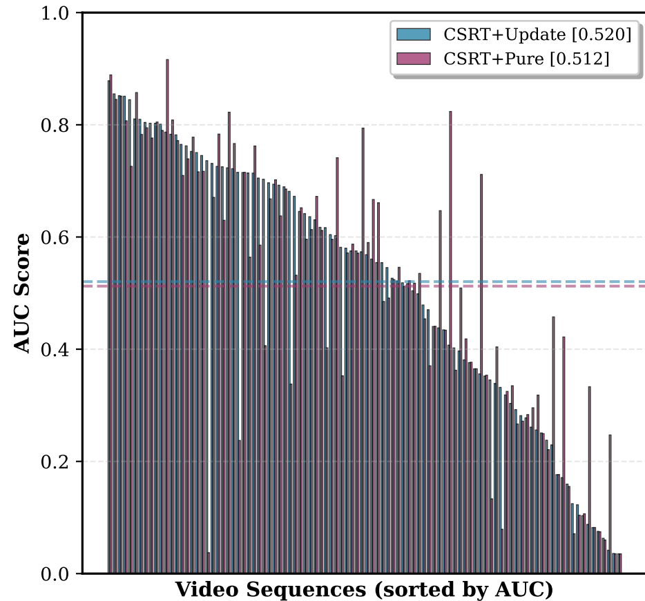
Success Plot - Area Under Curve
