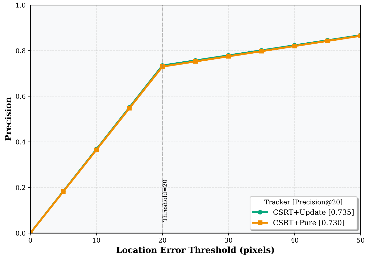
Precision Plot on OTB-100 Benchmark
