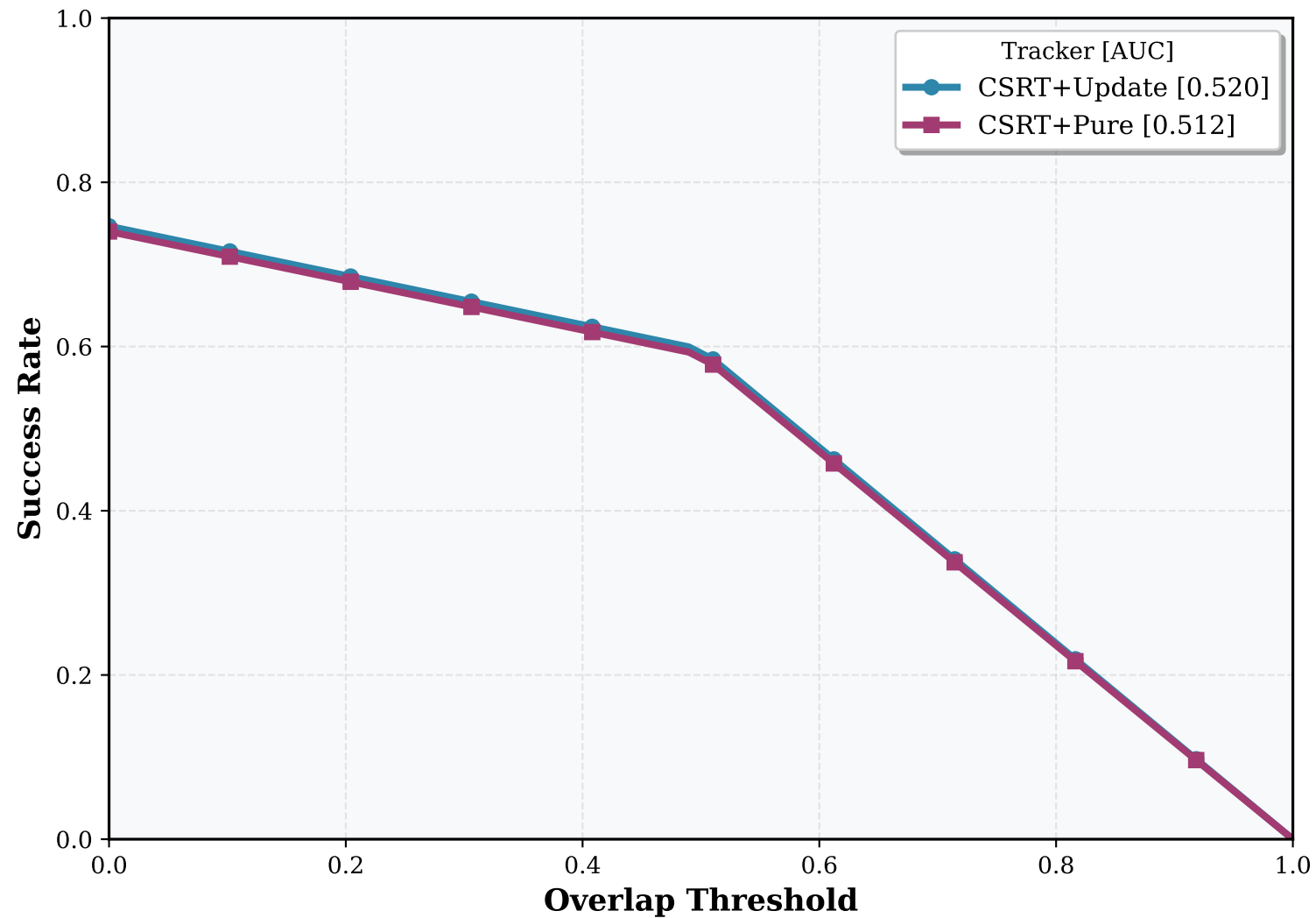
Success Plot on OTB-100 Benchmark
