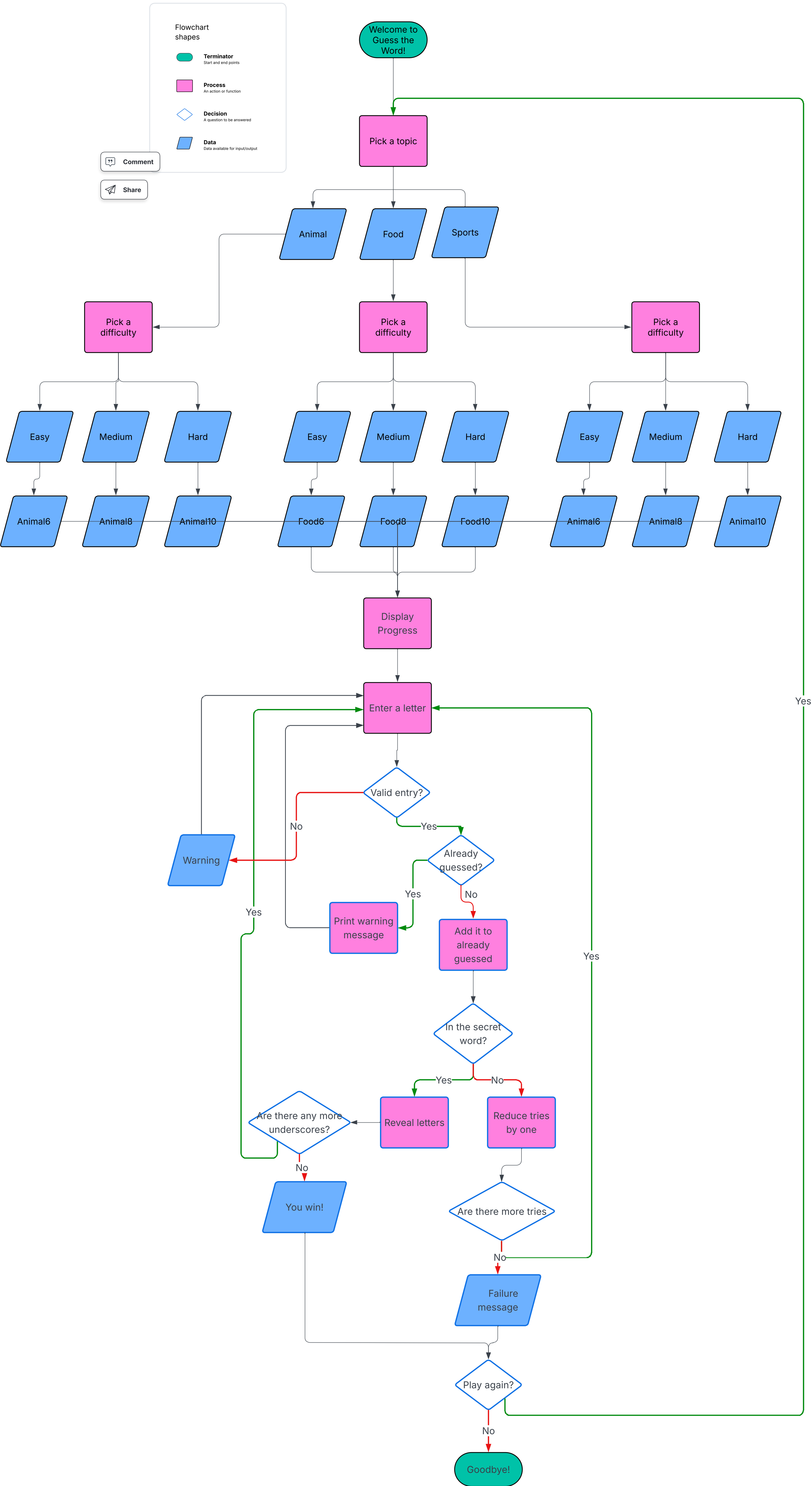
PA3 Guess the Word Flowchart
