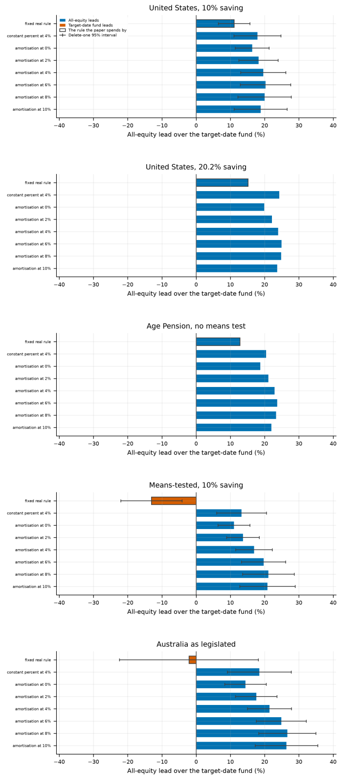
Figure 13. The all-equity portfolio's lead over the target-date fund, by pension system and withdrawal rule. One panel per system on a shared scale; the zero line is the ranking, the outlined bar is the rule the rest of this paper spends by, and the whiskers are delete-one-country 95% intervals where they were computed.
