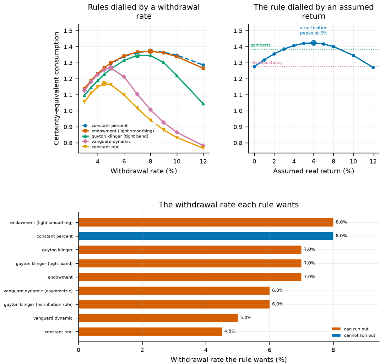
Figure 19. Where each dial that sets a spending level actually peaks. Top left, the certainty equivalent against the withdrawal rate for the five rules that take one; rings mark where each curve turns over, and solid lines can run out where dashed cannot. Top right, the same against the assumed real return for the rule dialled by one instead, with the two rules that set no dial at all drawn as the constant levels they are. A withdrawal rate and an assumed return are different measures, so they get an x-axis each; the vertical scale is shared between them, which is what lets the two peaks be compared by eye rather than by reading numbers off two ranges. Below, the withdrawal rate each rule wants.
