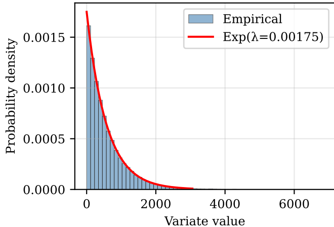
(a) Histogram vs Theoretical PDF
