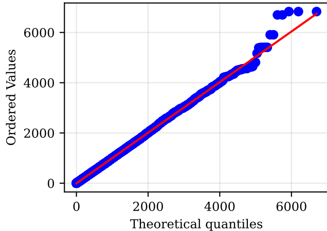
(b) Q-Q Plot
