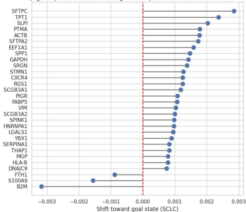
Top gene perturbations shifting LUAD epithelial cells toward SCLC state
