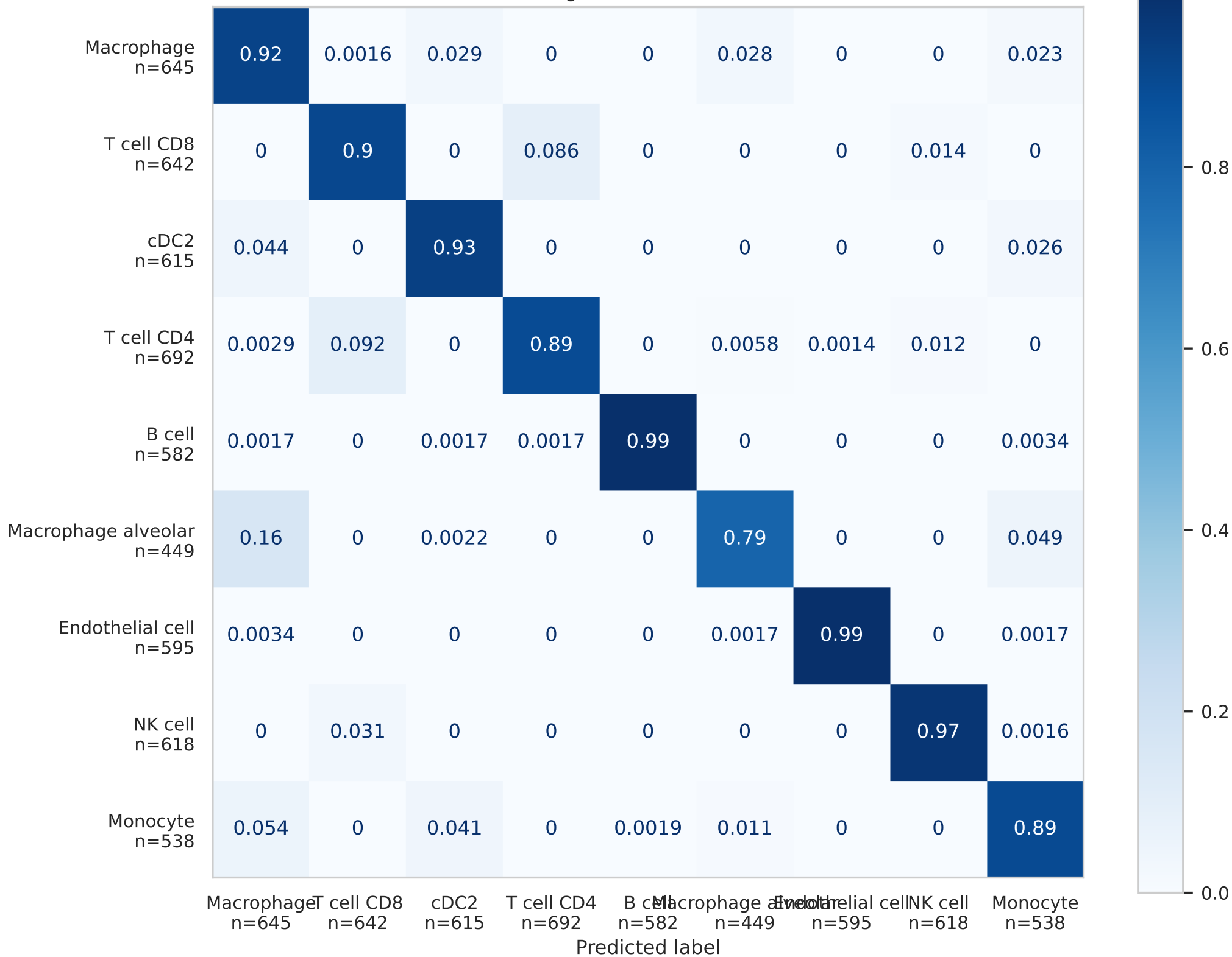
Stage 1 Geneformer V2
