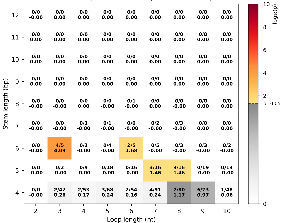
Loop excluding TC at the 3' end / Most stable hairpin
