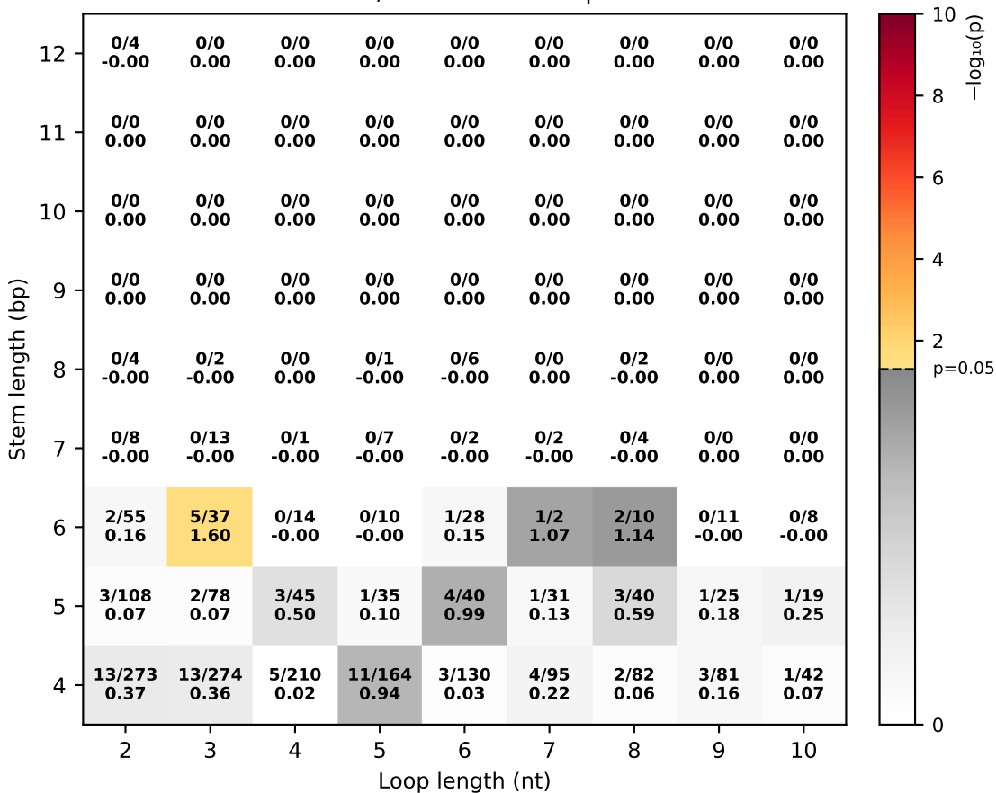
Stem / Most stable hairpin
