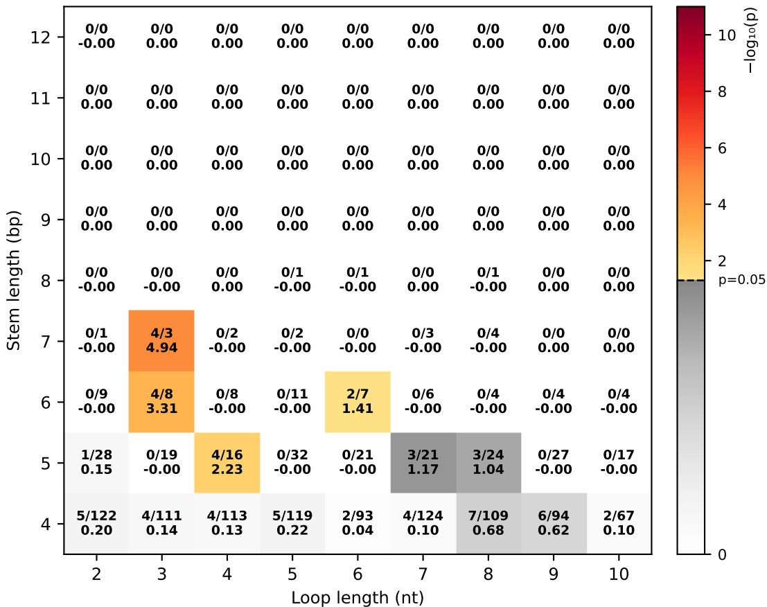
Hairpin loop / Most stable hairpin
