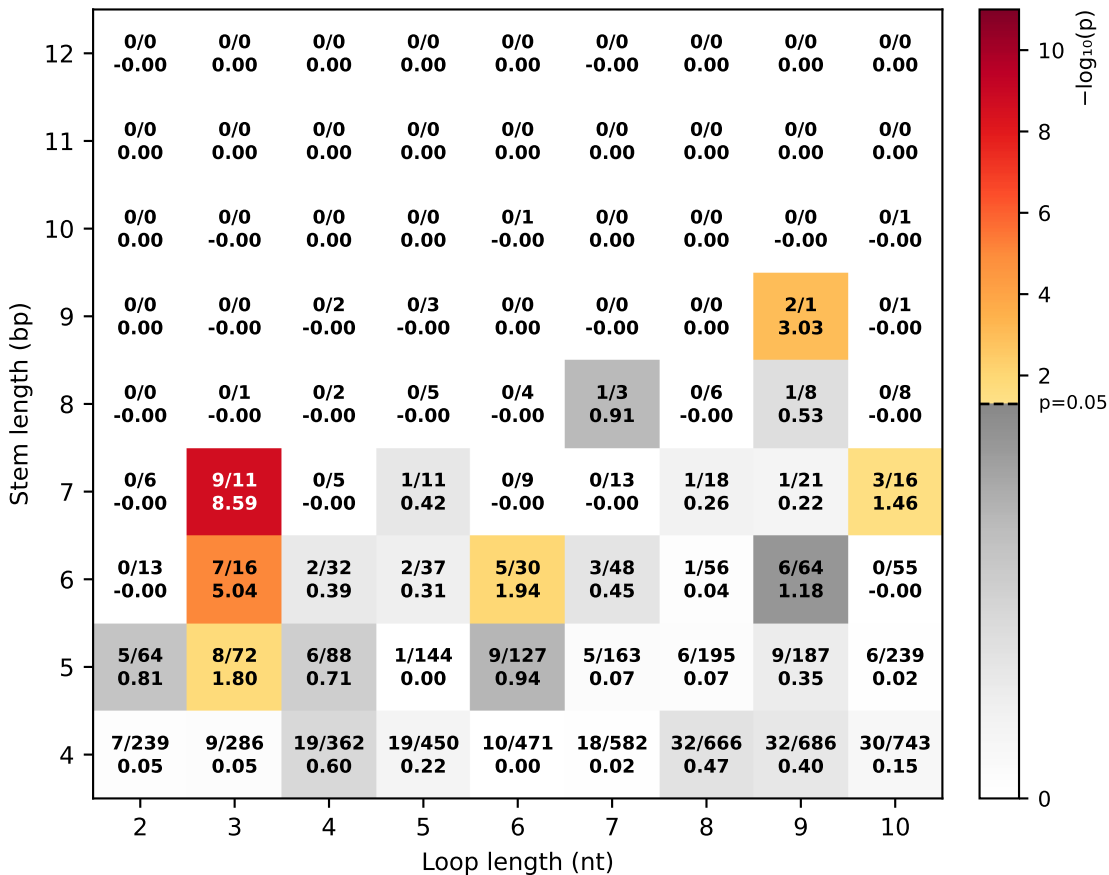
Hairpin loop / All hairpins
